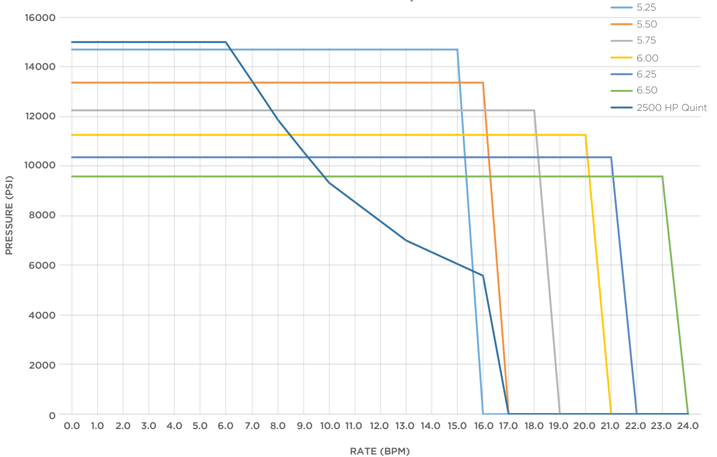
Durastim® Pump Curve
